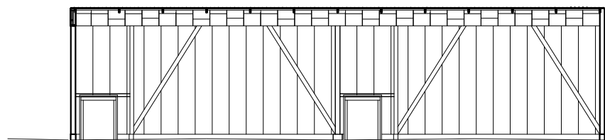
CORTE TRANSVERSAL H-H'
